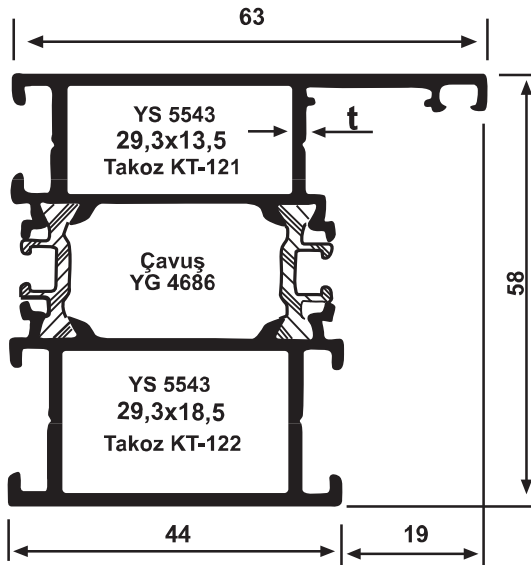
YS 5577/78 Kasa (t=2 mm) 1,735 kg/m YS 5577/78-B Kasa (t=1,5 mm) 1,580 kg/m
