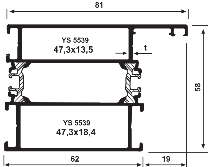
YS 5579/80 Geniş Kasa (t=2 mm) 2,105 kg/m
