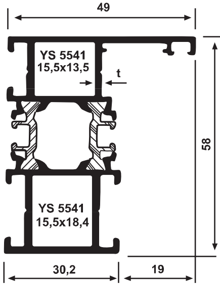
YS 5541/55 Dar Kasa (t=2 mm) 1,440 kg/m YS 5541/55-B Dar Kasa (t=1,5 mm) 1,325 kg/m
