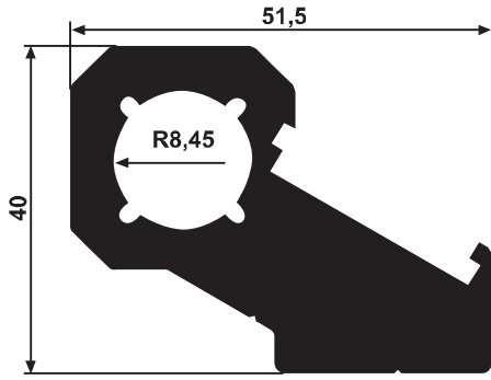
YG 1829 2,528 kg/m
