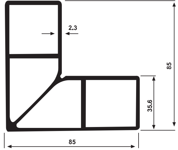
YG 4675 2,786 kg/m
